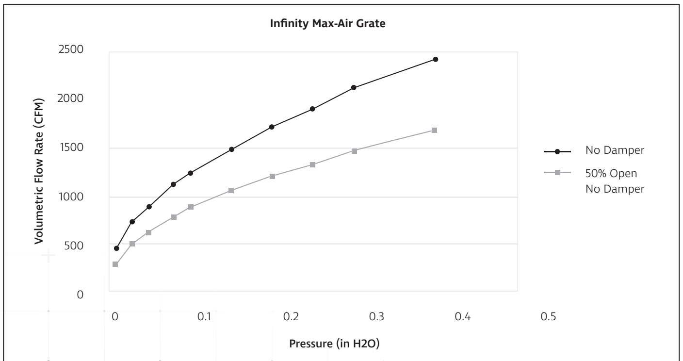
Figure 1 - Airflow Test Results
